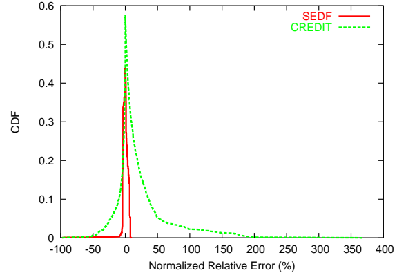
Figure 8: CDF_-^+ of CPU allocation errors.
