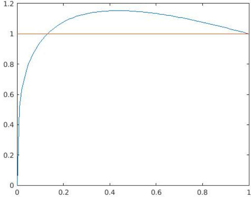
FIGURE 4. A graph of x^{p-1} + 2x^{(p-2)/2} - 2x^{p/2} (blue) and the constant 1 (red) for 0 \leq x \leq 1 .
