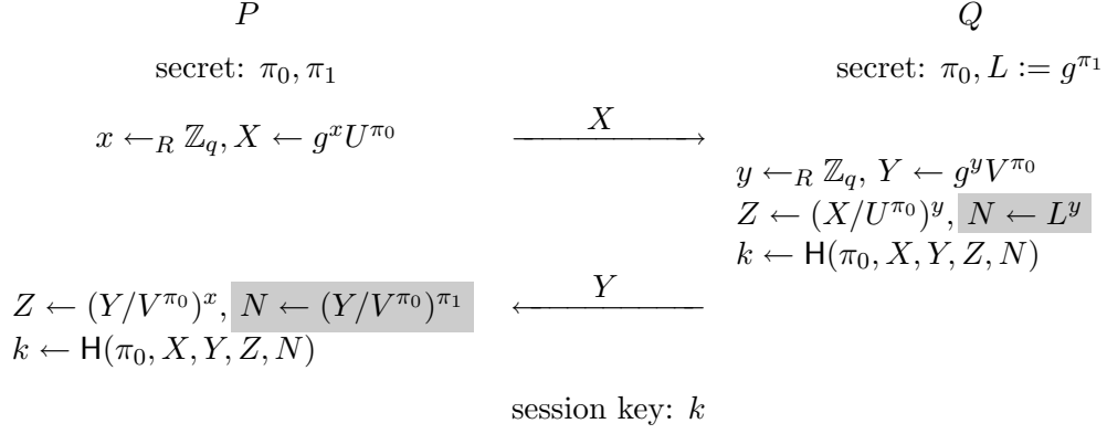
Figure 2: Protocol SPAKE 2 +
