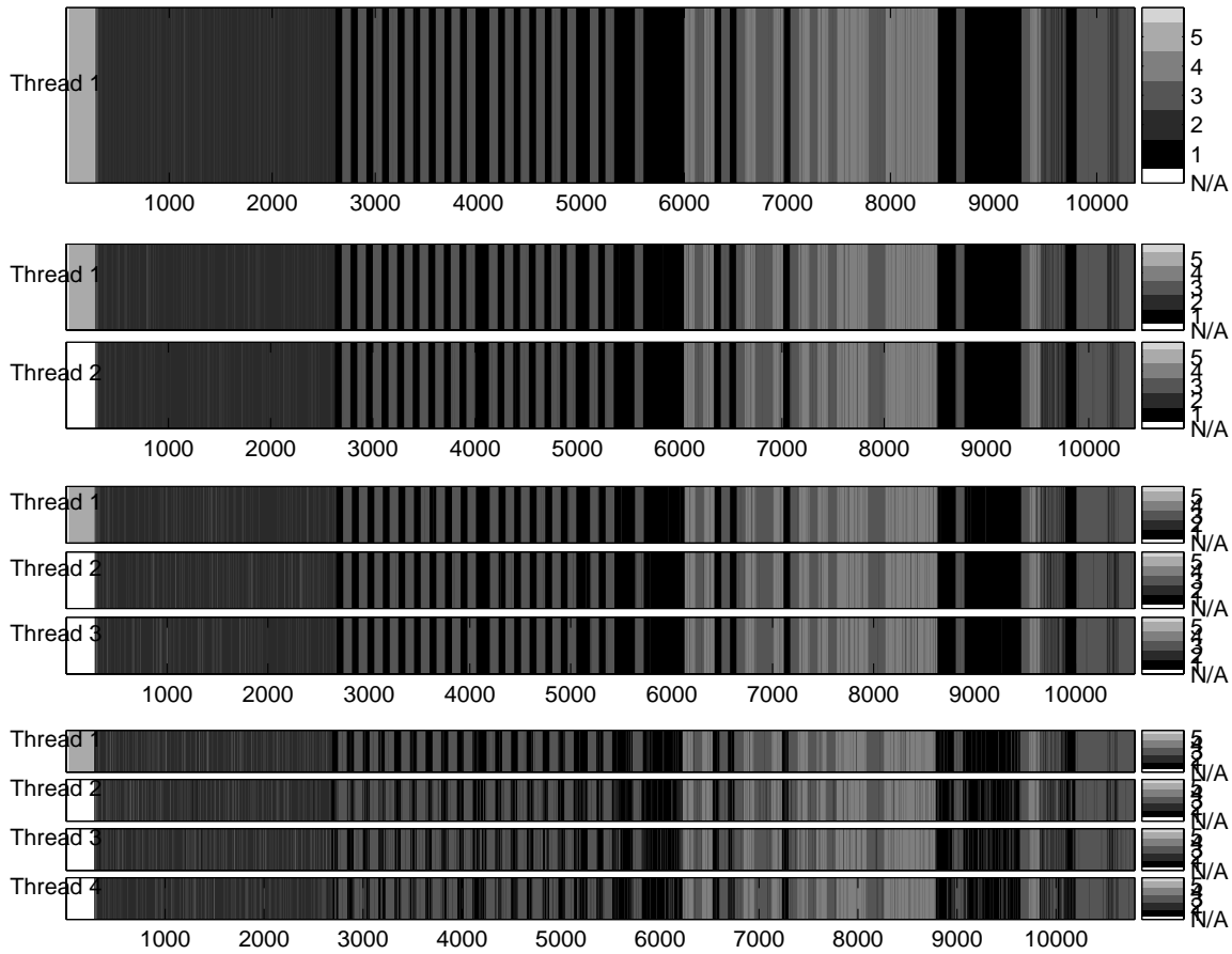
Figure 5: Phases discovered across 4 different parallel executions of snp : serial, 2, 3, and 4 threads. The x -axis shows the phase classification results over the global count of all instructions executed across all threads.
