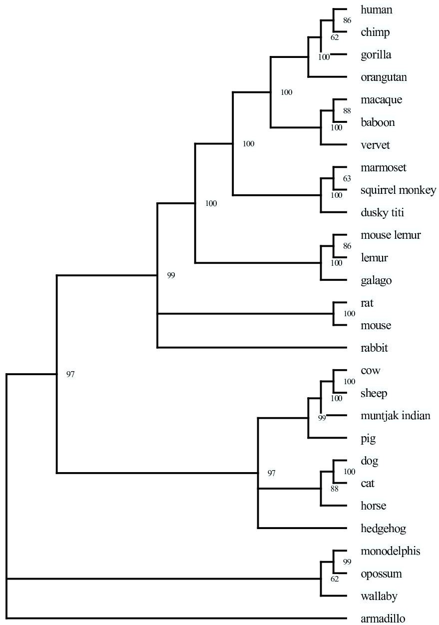
Figure 4: Phylogenetic tree of a large set of 28 species. Bootstrap support values are based on 1,000 bootstrap replicates. Tree image created using Treeview [24].
