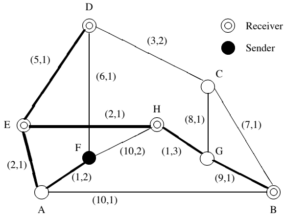
Figure 3. A Steiner multicast tree for this graph
