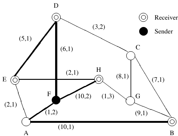
Figure 2. The multicast tree obtained by combining the separate optimal delay paths from the sender to each of the receivers
