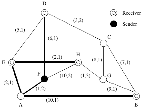
Figure 1. The multicast tree obtained by combining the separate optimal cost paths from the sender to each of the receivers
