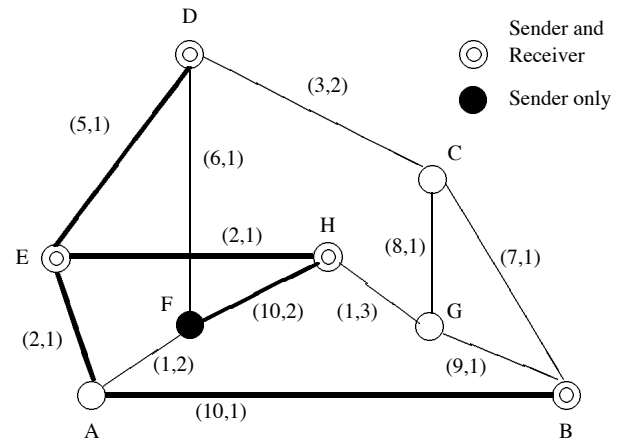
Figure 4. A core-based tree with node H as the core and optimal delay paths from the core to each receiver (this is a member-centered optimal-delay tree)
