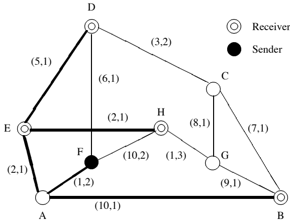
Figure 5. A Steiner tree with bounded maximum delay
