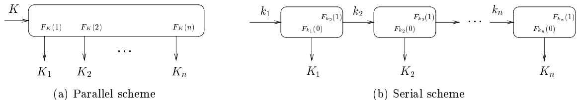
Figure 1: The parallel and serial re-keying schemes.
