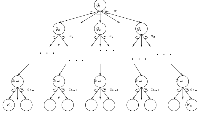
Figure 2: Diagram of our tree-based construction
