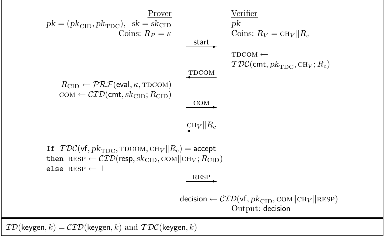
Figure 6: Reset-secure identification protocol ID for the CR1 setting based on an identification scheme CID secure against non-resetting CR1 attacks
