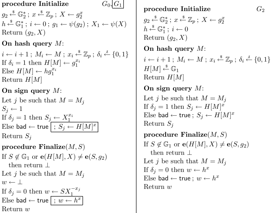
Figure 2.1: Games for the proof of Theorem 2.1. Game G_1 includes the boxed statements while G_0 does not.
