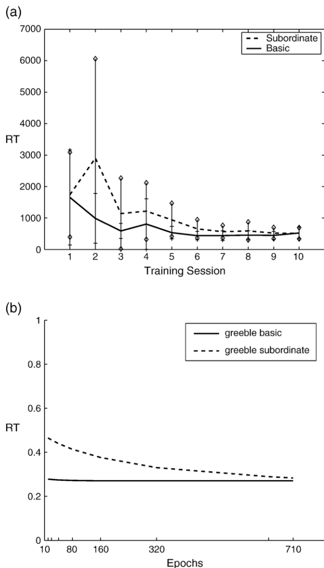
Fig. 5 – Entry level shift. (a) Typical reduction in reaction time for basic versus subordinate level judgments with training in a human subject learning to discriminate Greebles. (b) Reduction in reaction time in a neural network over training for subordinate versus basic level categorization. Reaction time is measured as the uncertainty of the maximum output ( 1 - \max_{\text{output}} ).
