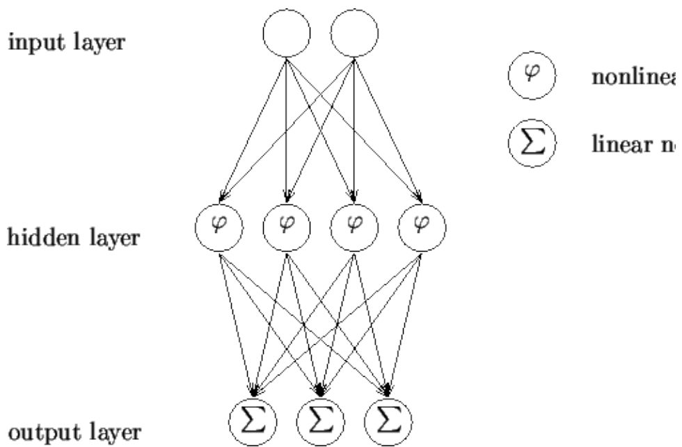
Figure 2: A multilayer perceptron with a single hidden layer. Picture from www.cis.hut.fi/ahonkela/dippa/ .
