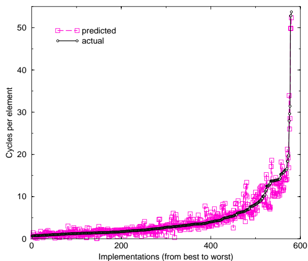
Figure 8: Predicting performance of matrix multiply with all terms through fourth-degree gives an R^2 of 93.6%. Using the 55 most important terms gives an R^2 of 92.5%.
