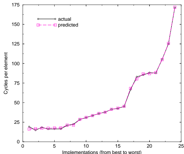
Figure 9: Predicting performance of FFT with all terms through second-degree gives a R^2 of 99.9%. Using only the five most important terms gives an R^2 of 98.37%.
