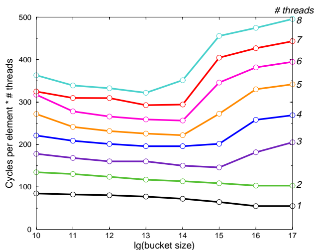
Figure 5: In integer sort, the best bucket size depends on number of threads.
