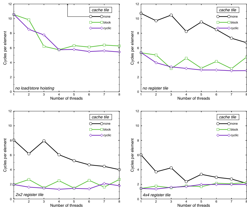
Figure 2: The best tuned matrix multiply, at 1.36 cycles per inner loop iteration, uses a 4 \times 4 register tile, a 32 \times 32 \times 32 cache tile, and two threads. With less tuning, more threads improves performance dramatically. As tuning increases, multithreading has less effect, eventually reducing performance.
