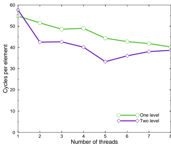
Figure 7: Comparison of two tilings of integer sort: two-level bucketing outperforms one-level bucketing.
