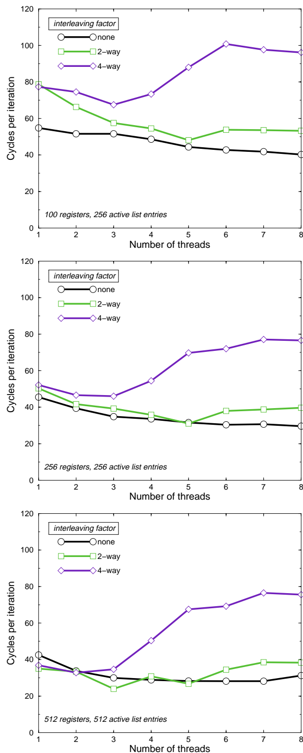
Figure 4: How much parallelism we can implement as ILP (via interleaving) depends on the availability of processor resources (number of rename registers and active list entries). Too much ILP with too few processor resources may overload the resources. TLP does not share this problem.
