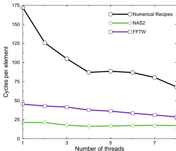
Figure 3: A comparison of three implementations of the Fast Fourier Transform on SMT.
