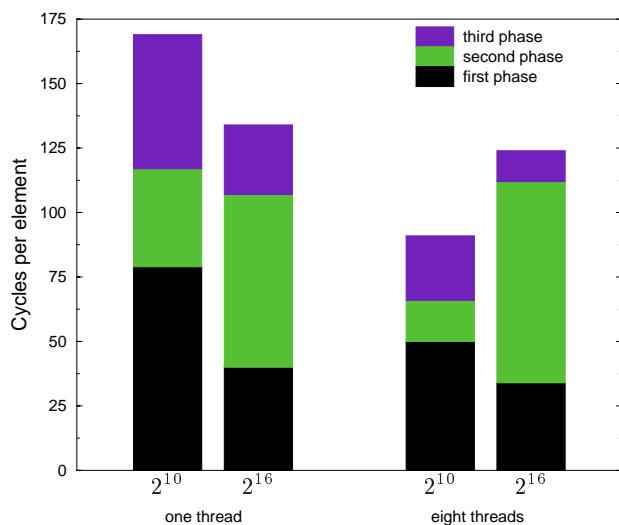
Figure 6: Increasing bucket size from 2^{10} to 2^{16} benefits the first and third phases of tiled integer sort, but harms the middle phase. This trade-off favors larger bucket sizes with fewer threads.
