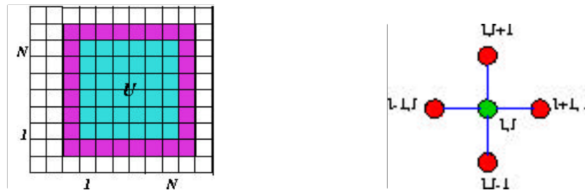
Figure 6a: A finite difference mesh (left) and the accompanying finite difference stencil (right). The Grid \mathbb{U} is defined over the 2-dimensional Region \text{domain}(0, 0, N+1, N+1) , i.e. the rectangle between lower bound (0, 0) and upper bound (N+1, N+1) . The solution is computed on the inner portion of the mesh; the boundary conditions are supplied on the outer edge. This boundary region is one cell thick, as dictated by the finite difference stencil for the smoother, which in our case updates each cell as a function of its nearest neighbors along the Manhattan directions.
