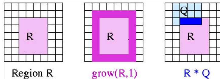
Figure 3b: Examples of Region calculus operations grow and intersection * . Q and R are regions. grow(R, 1) expands the Region R by one unit in all directions, and is commonly used to grow a halo region for stencil computations. We can intersect this halo region with the other subdomain to determine data dependencies requiring communication
