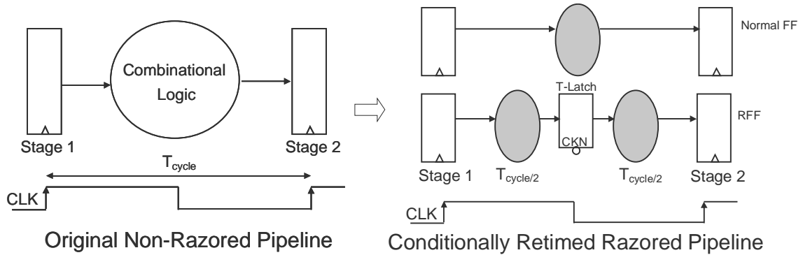
Figure 6.1 Latch-insertion scheme for satisfying the short-path constraint
