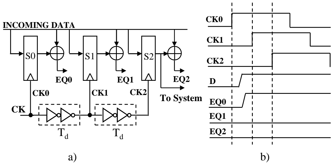
Figure 2.2 Kehl's triple-latch technique for in situ delay monitoring. Figure a) shows the mechanism of monitoring delay through temporal redundancy. Figure b) shows the timing diagrams for a “tuned” system
