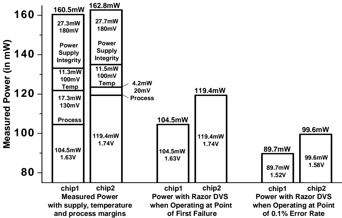
Figure 4.6 Total Energy Savings with RazorI.
