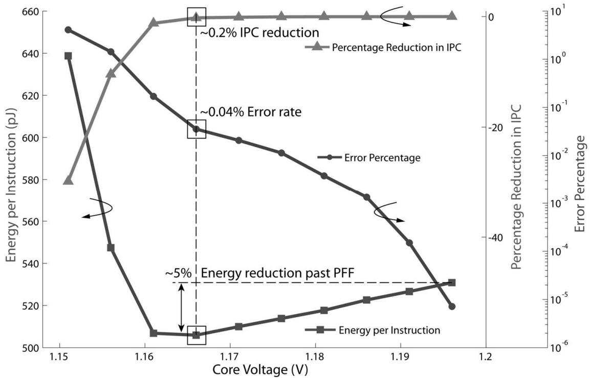
Figure 7.8 Sub-critical operation in RazorII
