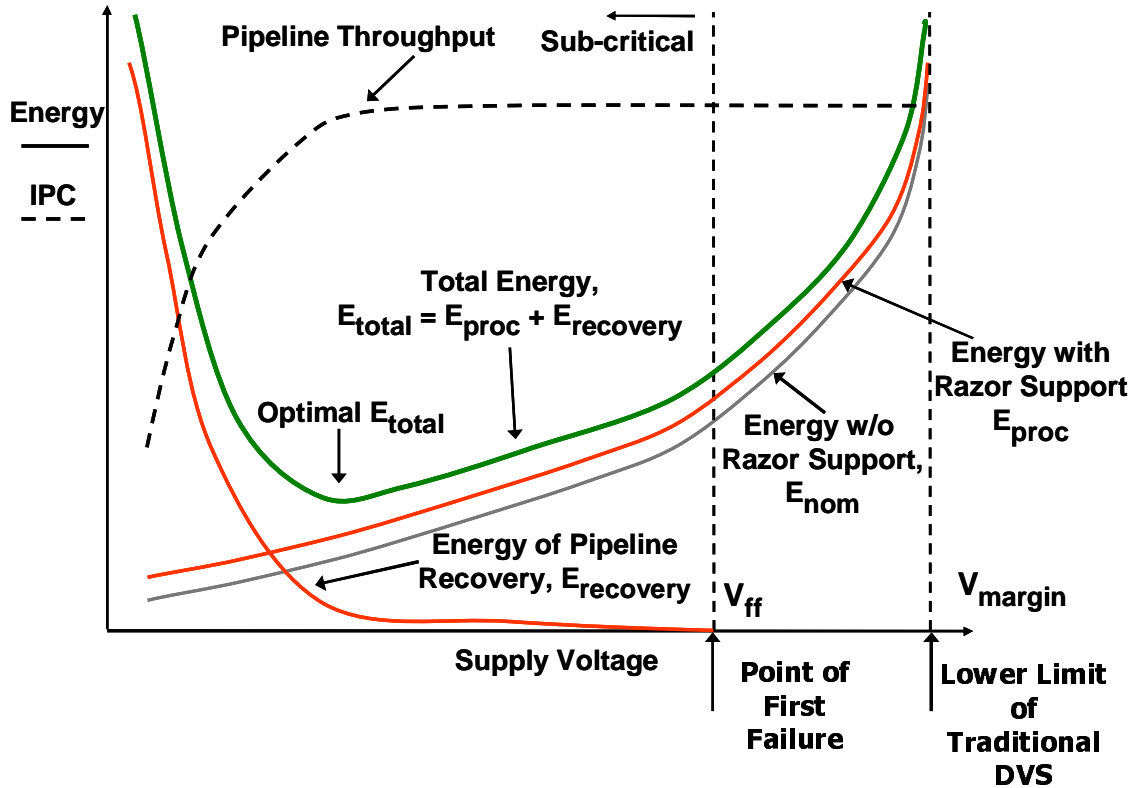
Figure 1.2 Qualitative relationship between supply voltage and Error-rate
