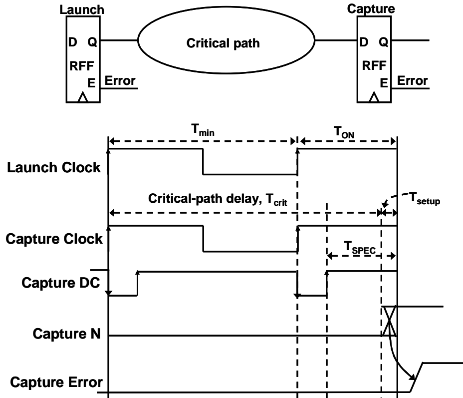
Figure 7.2 The limit of safe operation in RazorII
