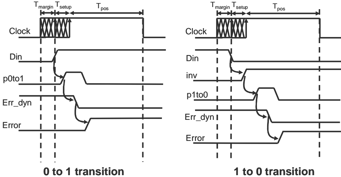
Figure 5.5 Timing diagrams showing the principle of operation of the Transition Detector
