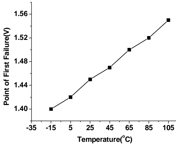
Figure 4.5 Temperature margins
