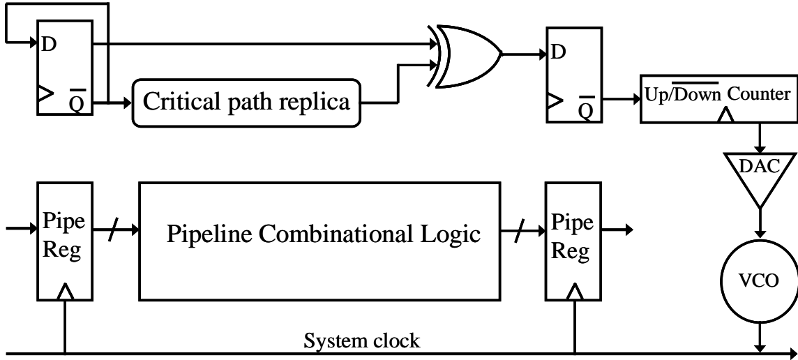
Figure 2.1 Uht's TEATime: A canary circuits based approach
