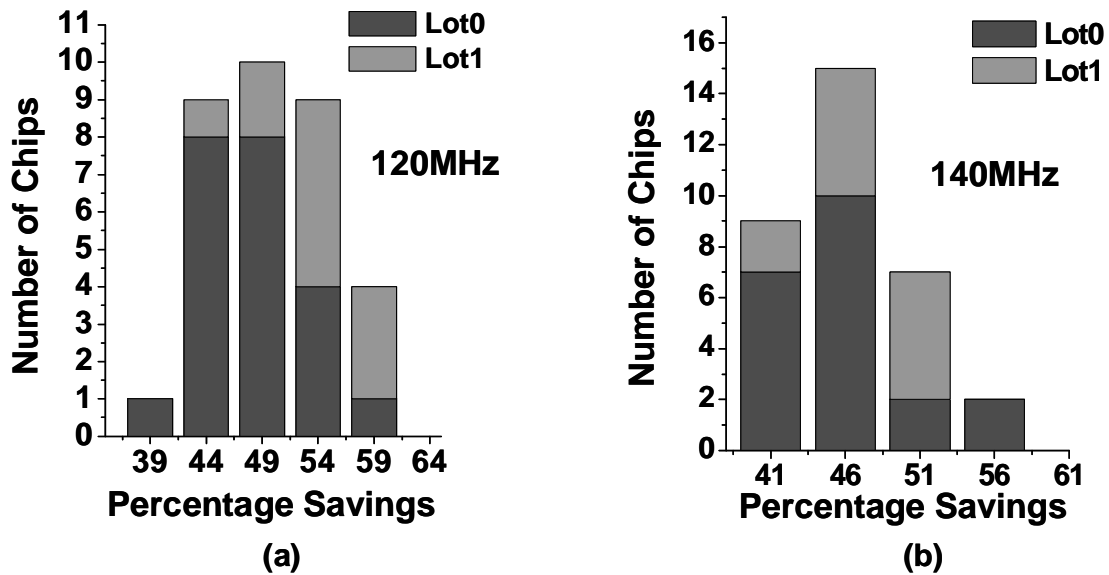
Figure 4.7 Distribution of the total energy savings over the worst-case for 33 measured chips.
