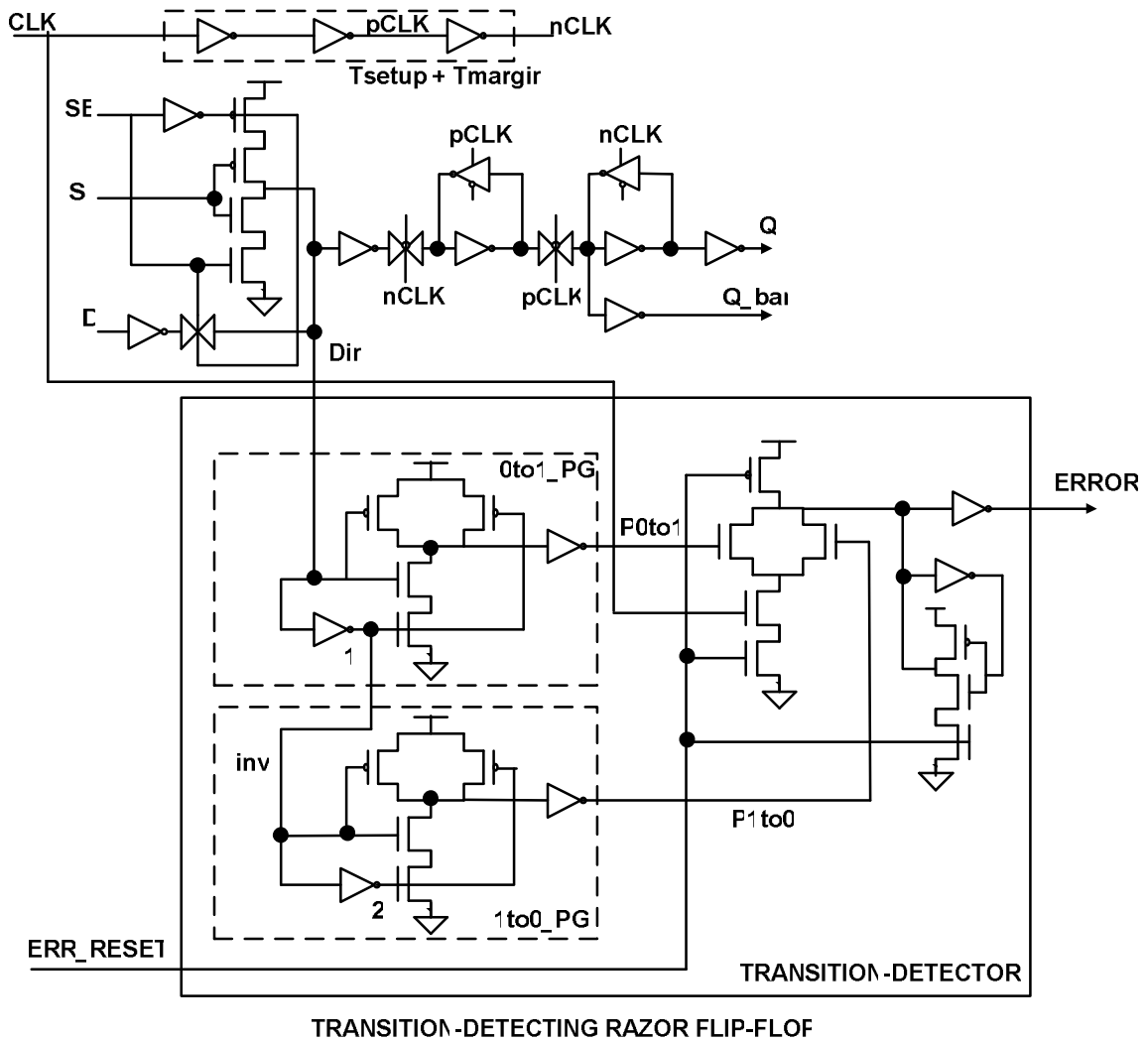
Figure 5.4 Transition-detecting RazorII flip-flop
