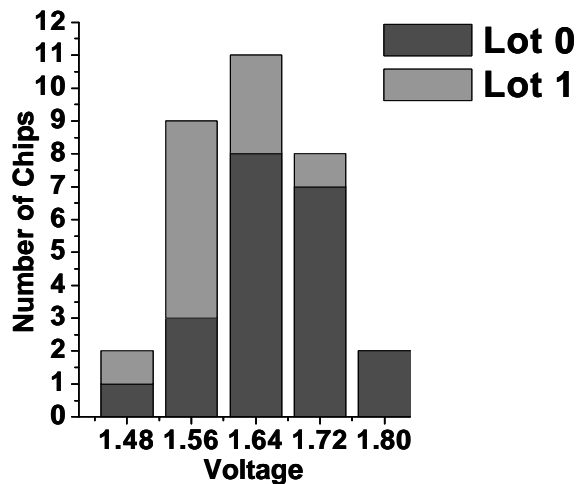
Distribution of Point of First Failure (a)
