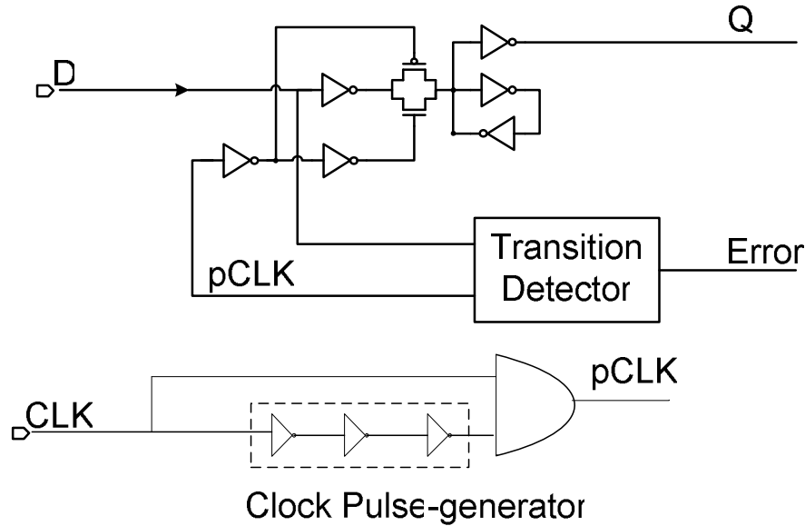
Figure 6.5 Pulsed-latch implementation of the RazorII flip-flop. The transition-detector monitors the data input rather than the internal node.
