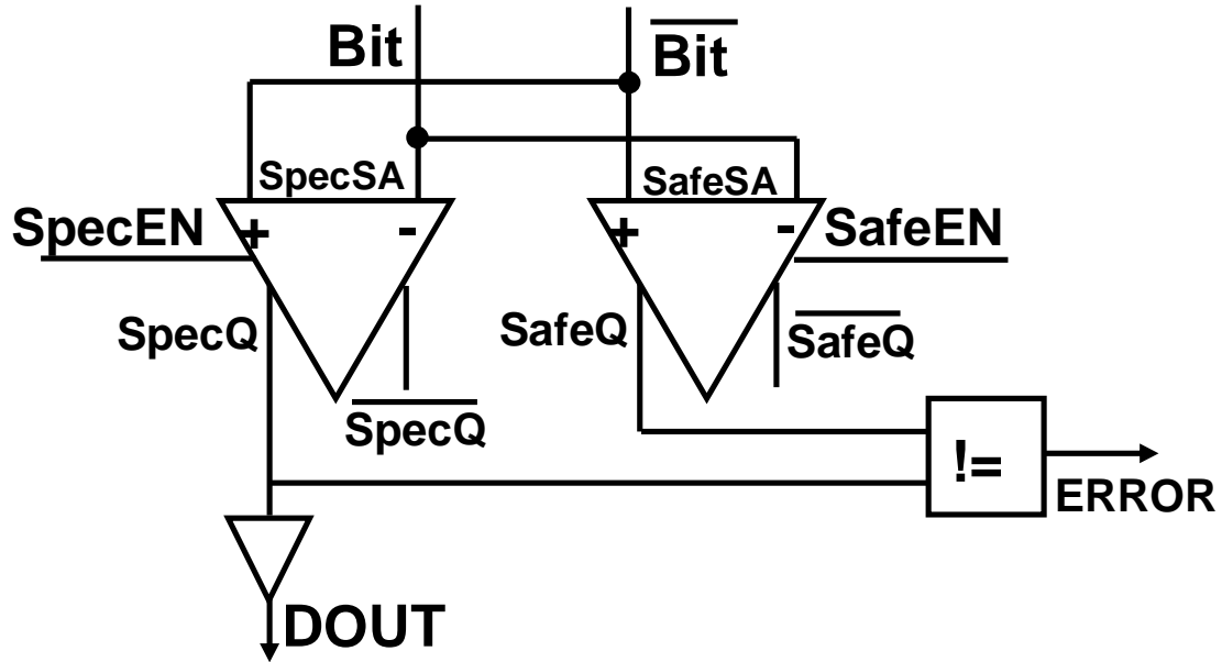
Figure 5.12 Dual Sense-amplifier scheme for faster read timings
