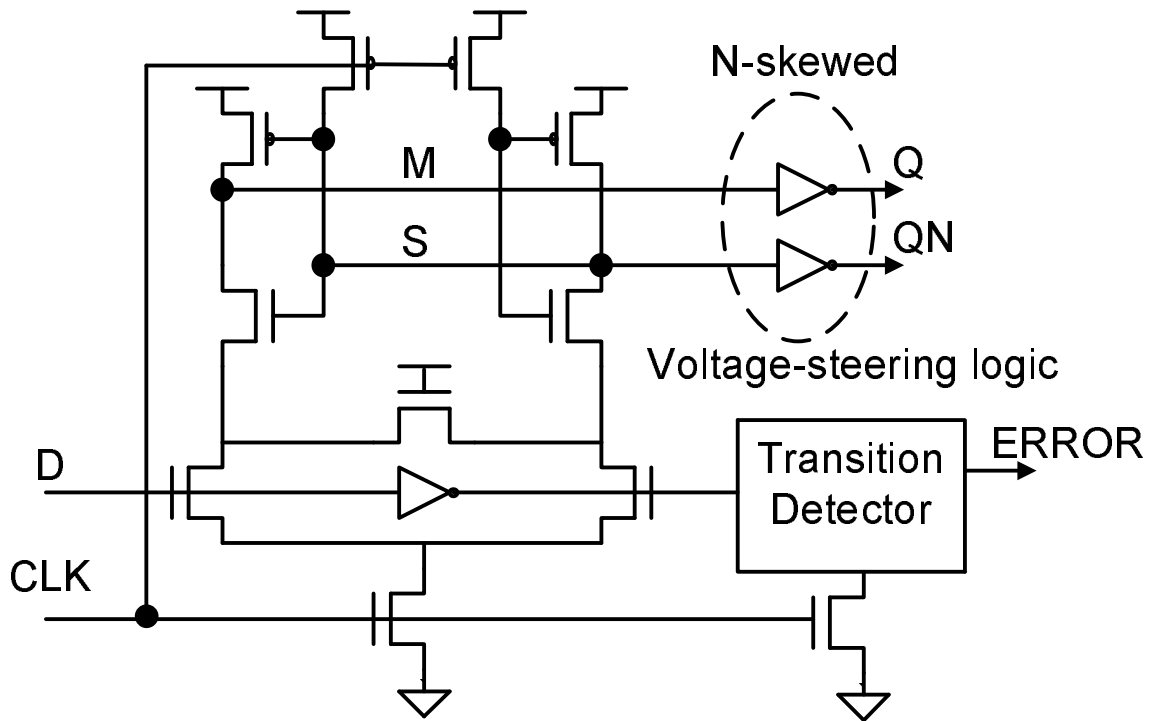
Figure 5.11 Sense-amplifier Flip-flop augmented with a transition-detector to sample critical Read signals in a SRAM array
