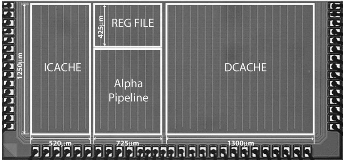
Figure 7.4 Die-photograph of the RazorII processor
