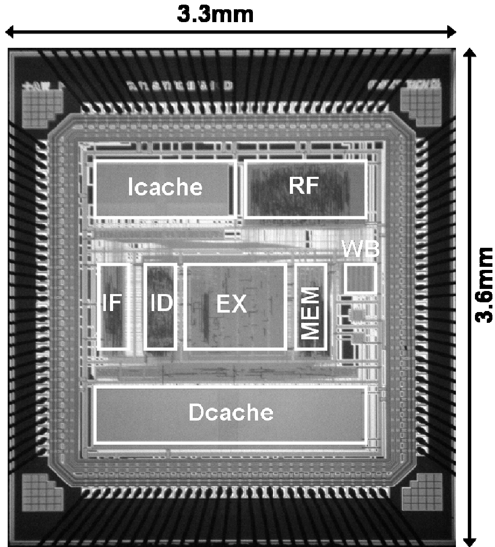
Figure 4.1 Die photograph of the RazorII processor. The 64bit processor executes a sub-set of the ALPHA instruction set.
