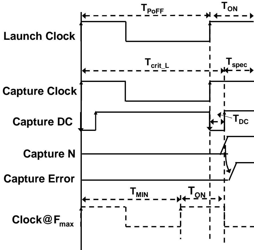
Figure 7.3 Worst-case vector based tuning
