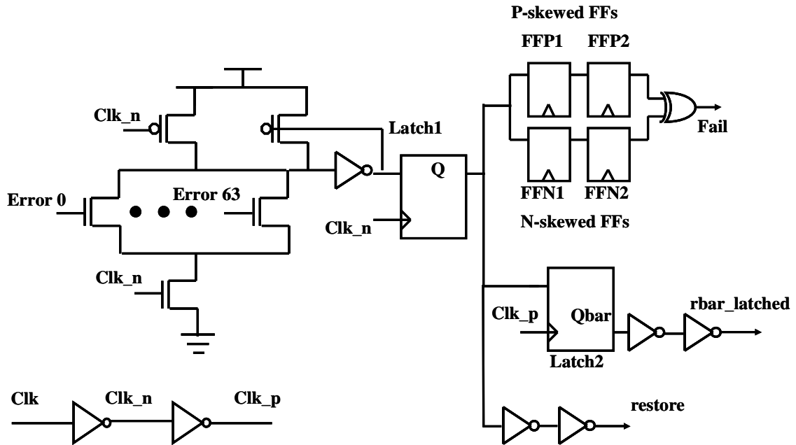
Figure 3.4 Restore generation circuitry
