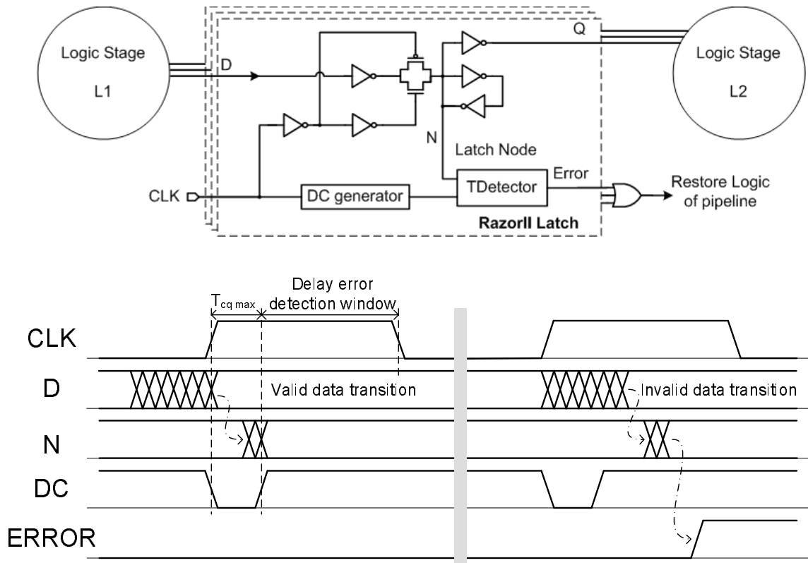
Figure 5.6 Modified RazorII flip-flop for SEU and timing-error detection
