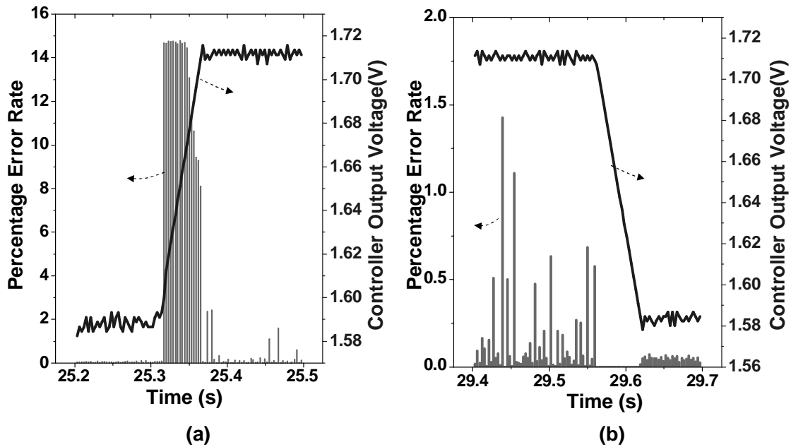
Figure 4.10 RazorI voltage controller: Error-rate phase transition response. Figure a) shows the transition from low to high error-rate. Figure b) shows the transition in the opposite direction.
