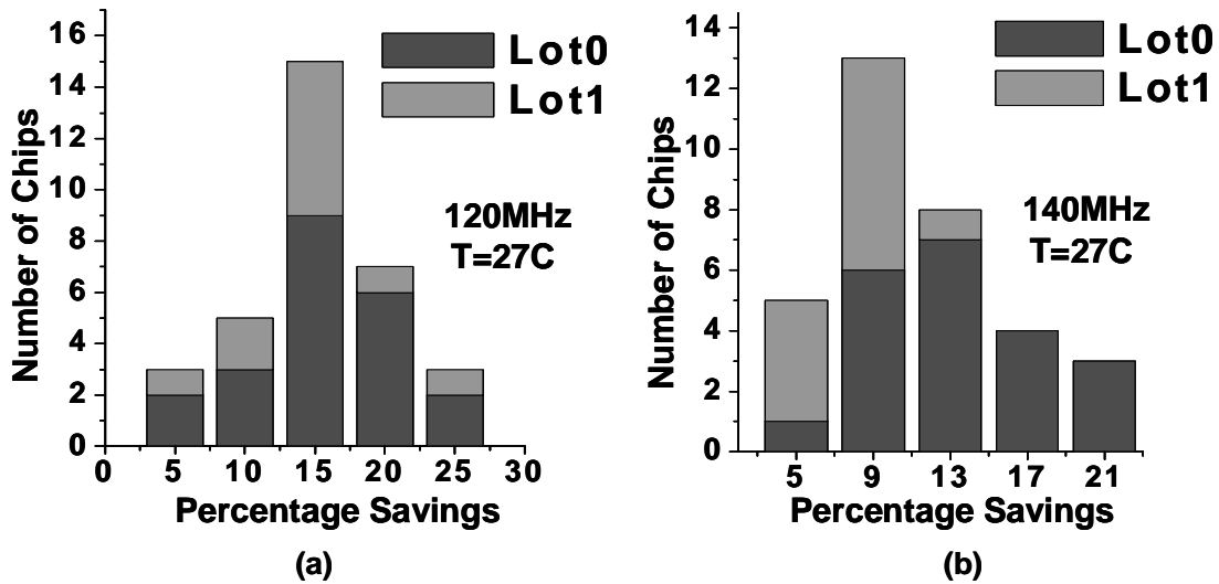
Figure 4.3 Normalized energy savings over point of first failure at the 0.1% error-rate for 33 measured chips at 120 and 140MHz.
