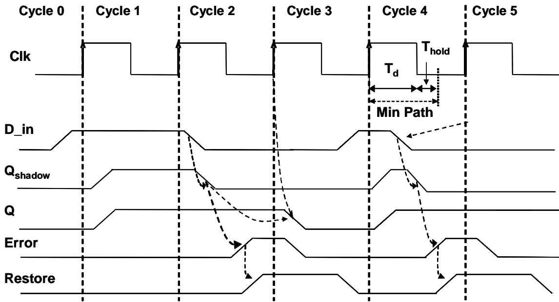
Figure 3.2 Conceptual timing diagrams showing the operation of the RazorI flip-flop. In Cycle 2, a setup violation causes Error to be flagged whereas in Cycle 4, a hold violation causes error to be asserted.
