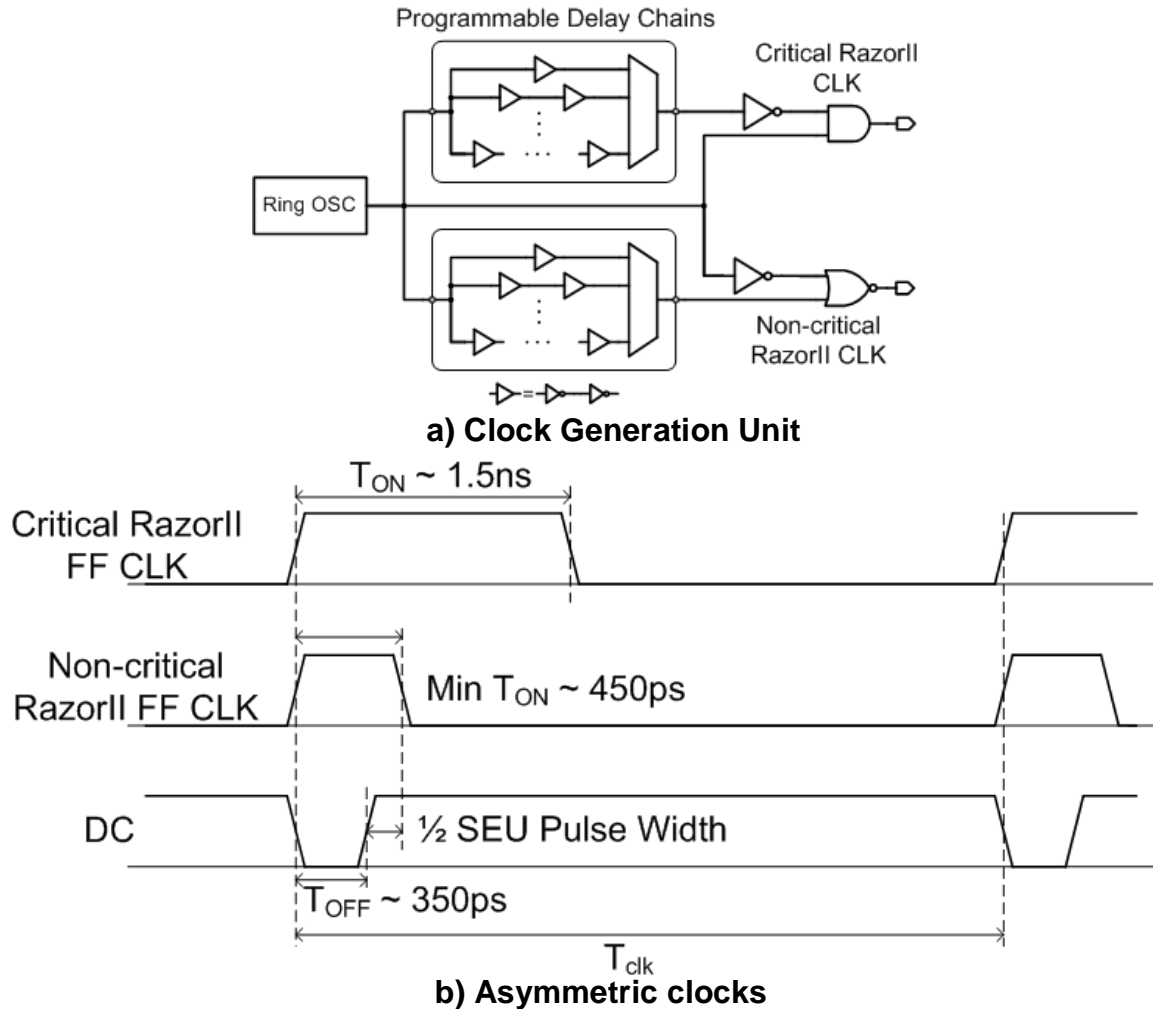
Figure 7.5 RazorII processor clocking scheme. Figure a) shows the schematic of the clock-generator. Figure b) shows the relevant timing diagrams.
