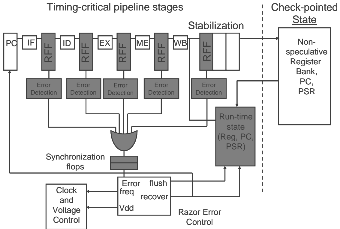
Figure 5.2 RazorII pipeline organization
