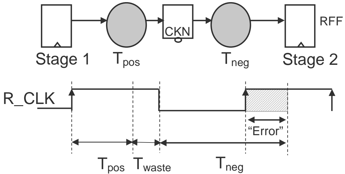
Figure 6.2 Error-rate and wasted-time trade-off
