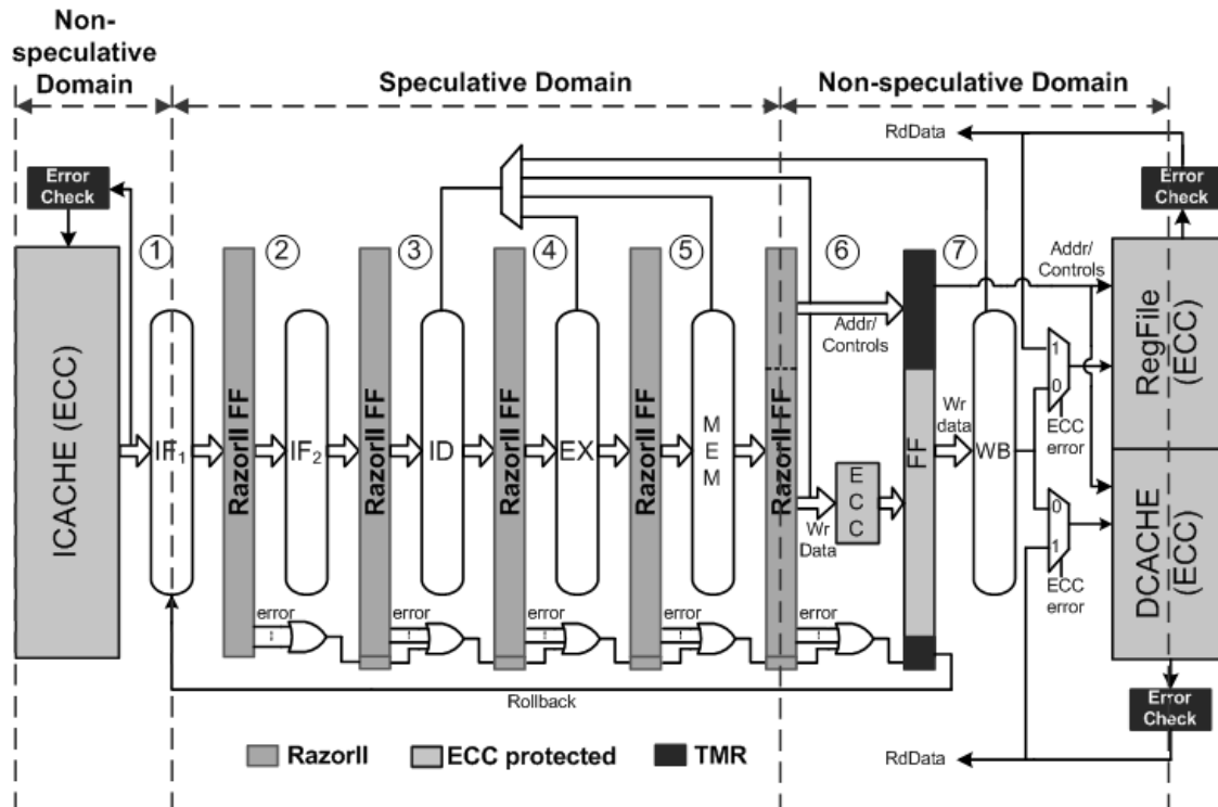
Figure 7.1 RazorII Processor: Pipeline Design
