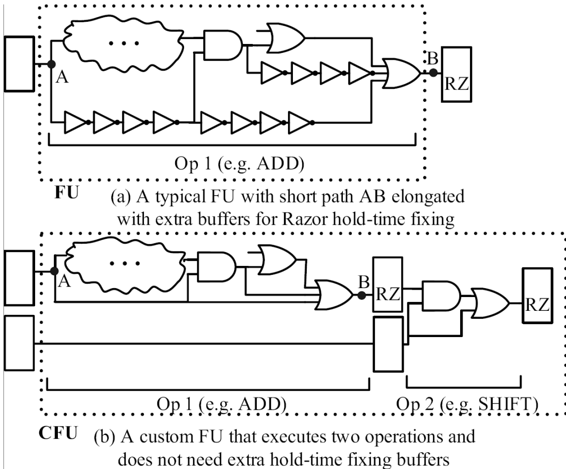
Figure 6.4 Replicated functional units eliminate the Razor minimum-delay constraint
