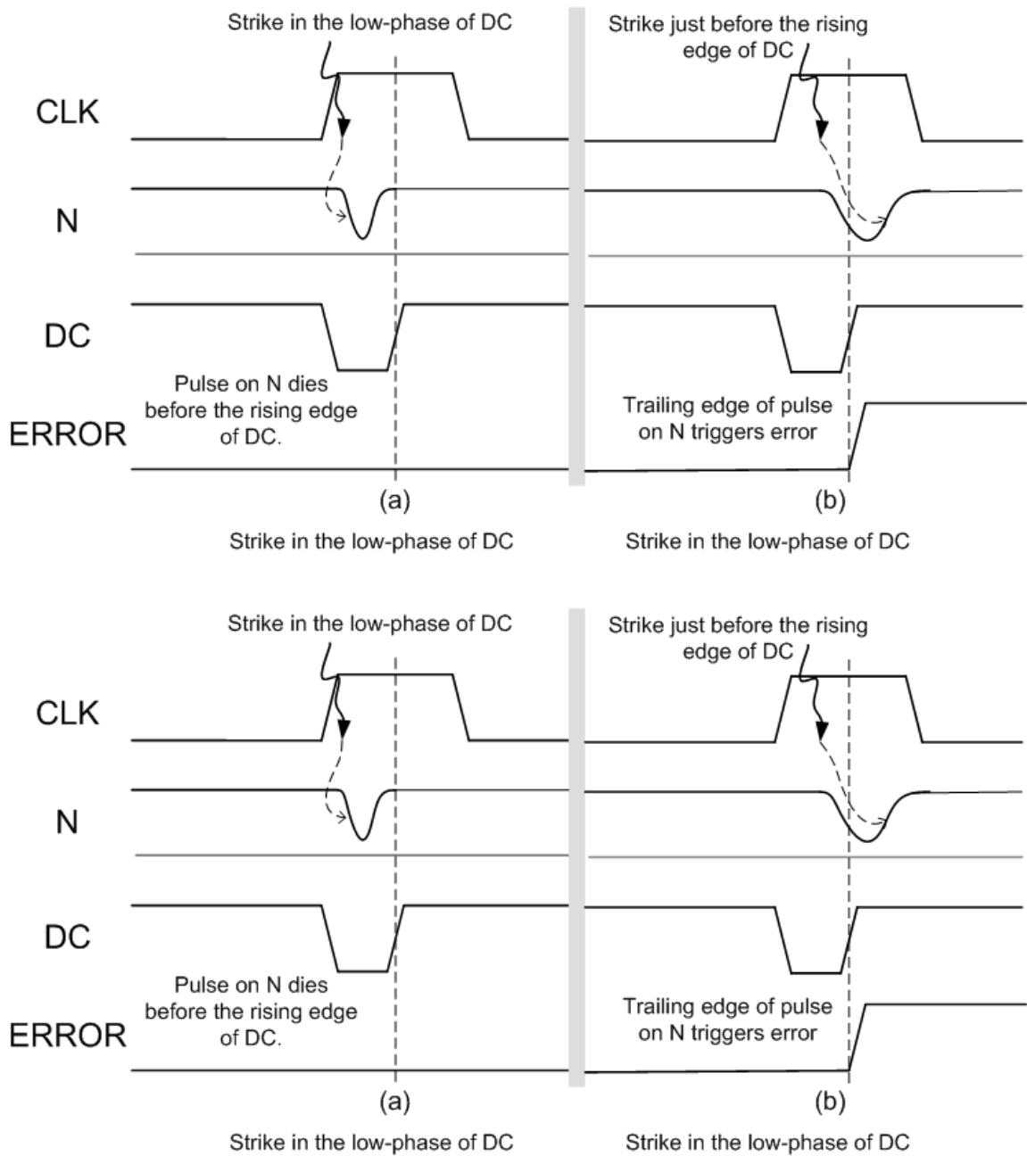
Figure 5.10 SEU Detection when DC pulse is low
