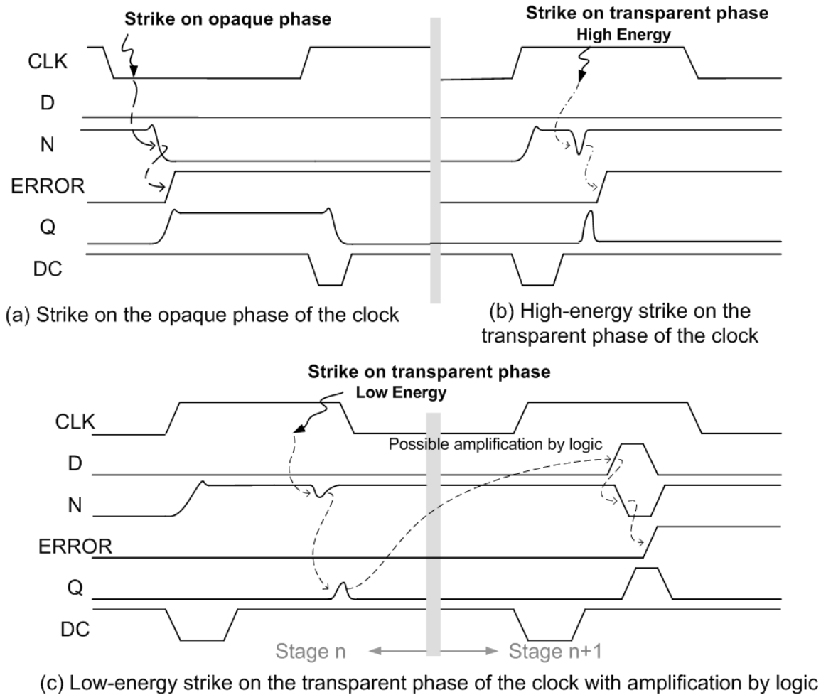
Figure 5.9 Conceptual timing diagrams showing SEU detection when DC is high
