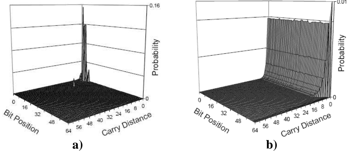
Figure 2.3 Data-dependent delay variations in adders a) Carry-propagation for SPECInt 2000 vectors b) Carry-propagation for random vectors [25]
