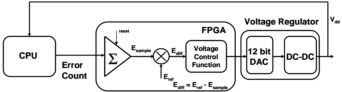
Figure 4.8 RazorI voltage control loop
