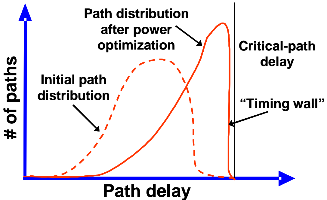
Figure 1.1 Timing wall: A consequence of downsizing off-critical paths [40]
