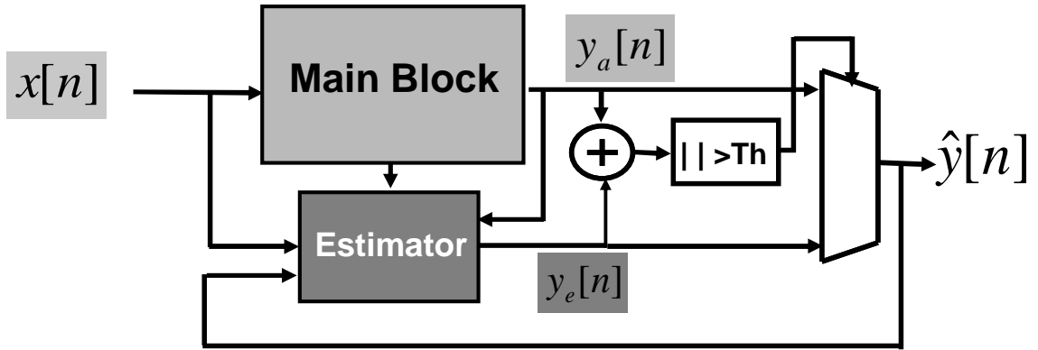
Figure 2.5 Algorithmic Noise Tolerance [30]
