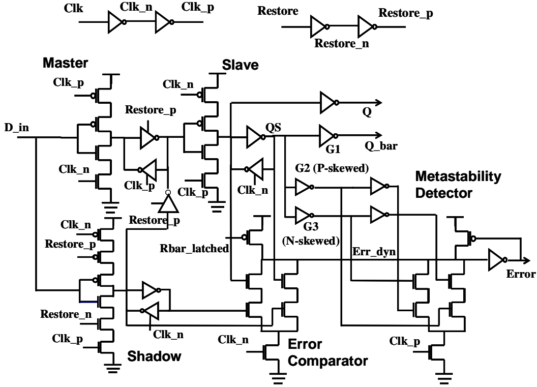
Figure 3.3 RazorI flip-flop circuit schematic
