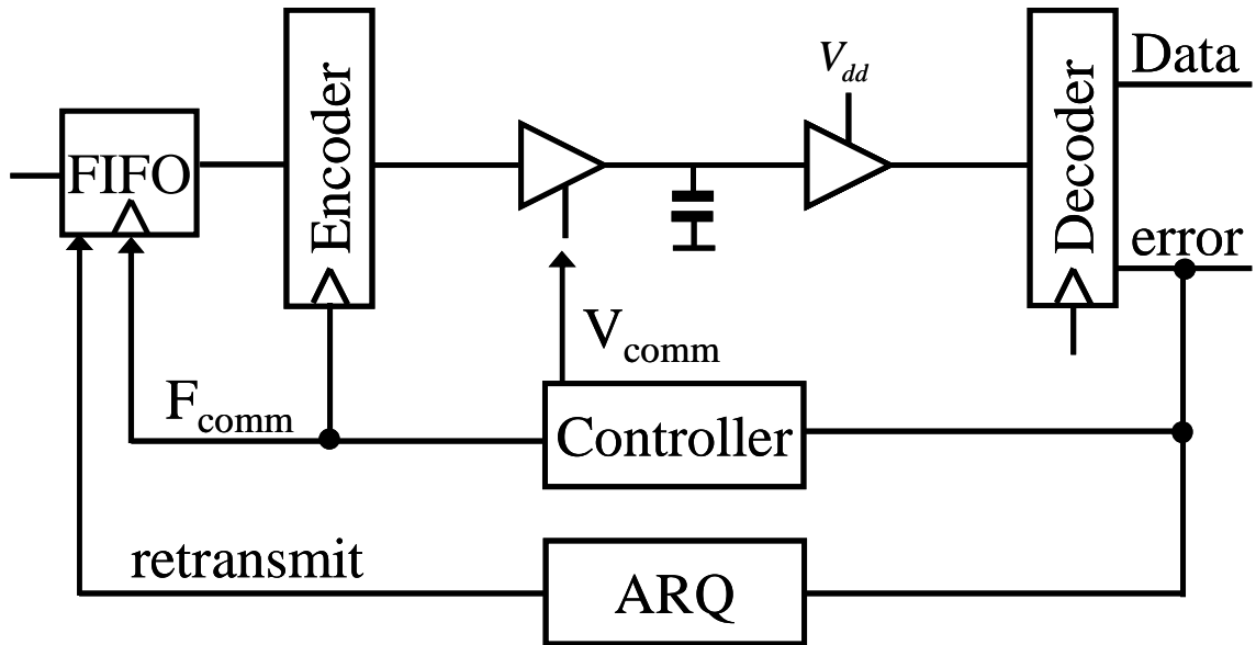
Figure 2.4 Self-calibrating interconnects
