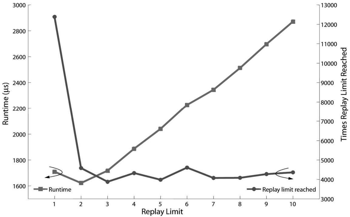
Figure 7.9 Run-time versus replay tradeoff
