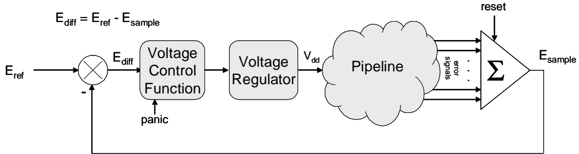
Figure 3.8 Razor supply voltage control
