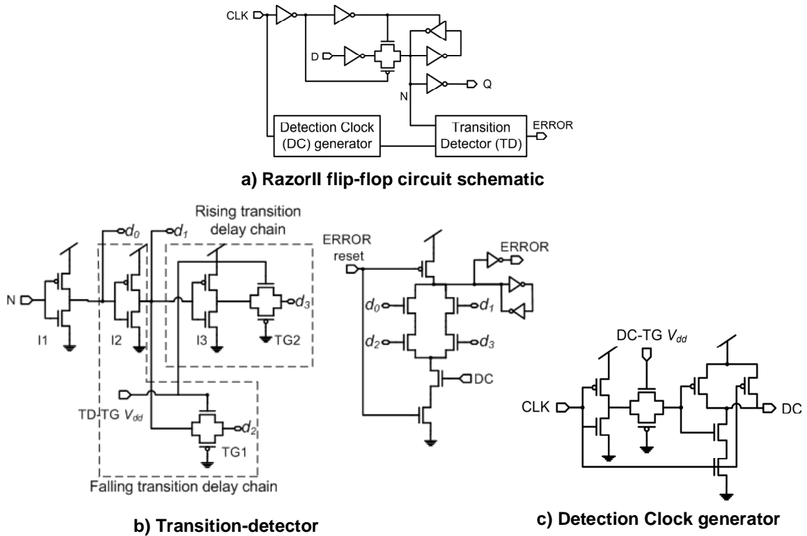
Figure 5.7 Circuit schematic of the R2LAT
