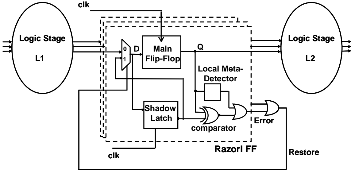
Figure 3.1 Abstract view of the RazorI flip-flop. The speculative data in the master-slave flip-flop is compared with the correct data in the positive level-sensitive shadow latch.
