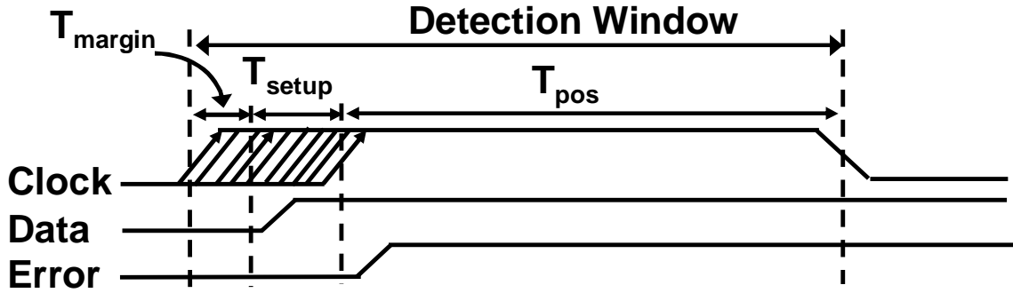
Figure 5.3 Transition-detection based error detection
