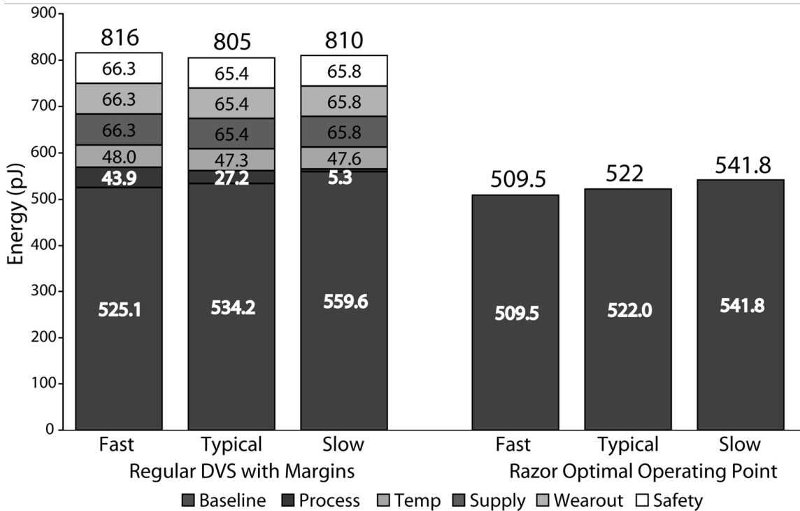
Figure 7.6 Total energy savings through RazorII based supply-voltage control
