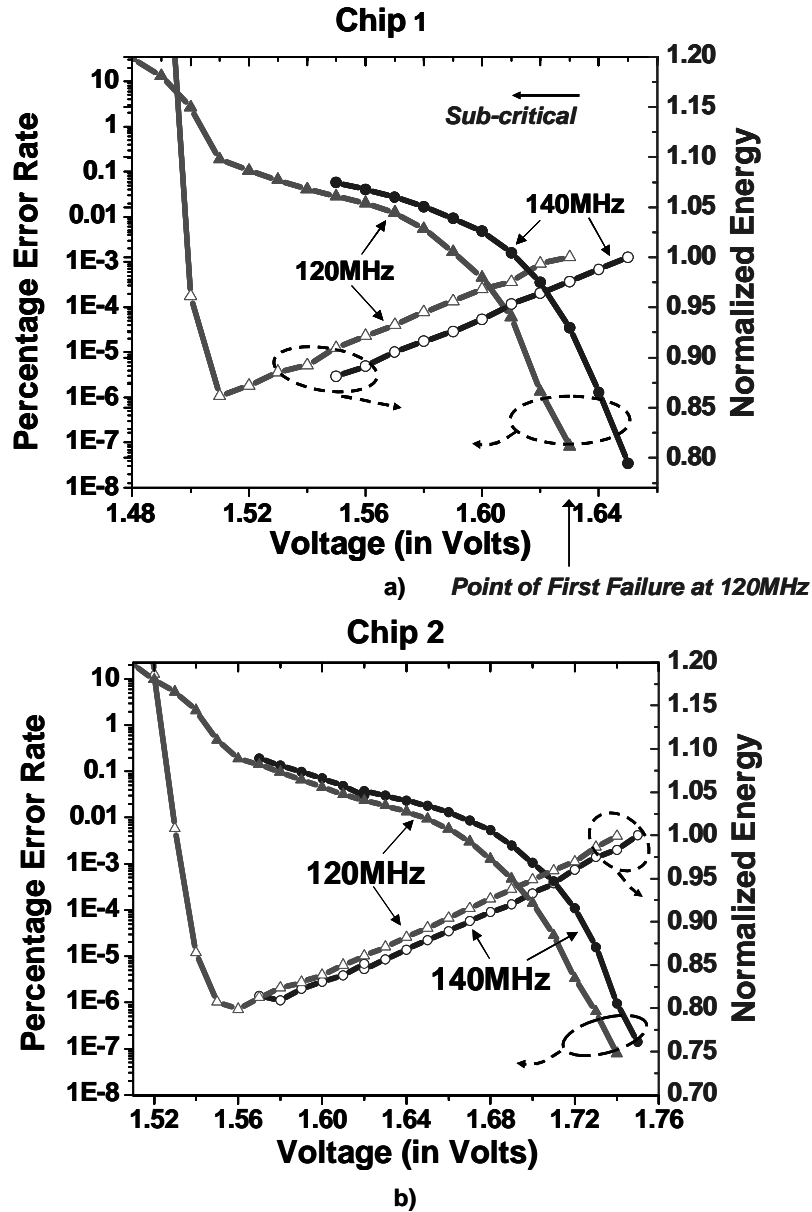
Figure 4.2 Sub-critical operation in chips named "Chip 1" and "Chip 2"
