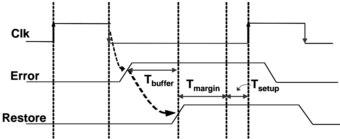
Figure 5.1 Timing constraint on the Restore signal. The Restore signal is a high fan-out net which is generated out of a high fan-in OR gate. It needs to setup before the next rising edge with sufficient safety margin.
