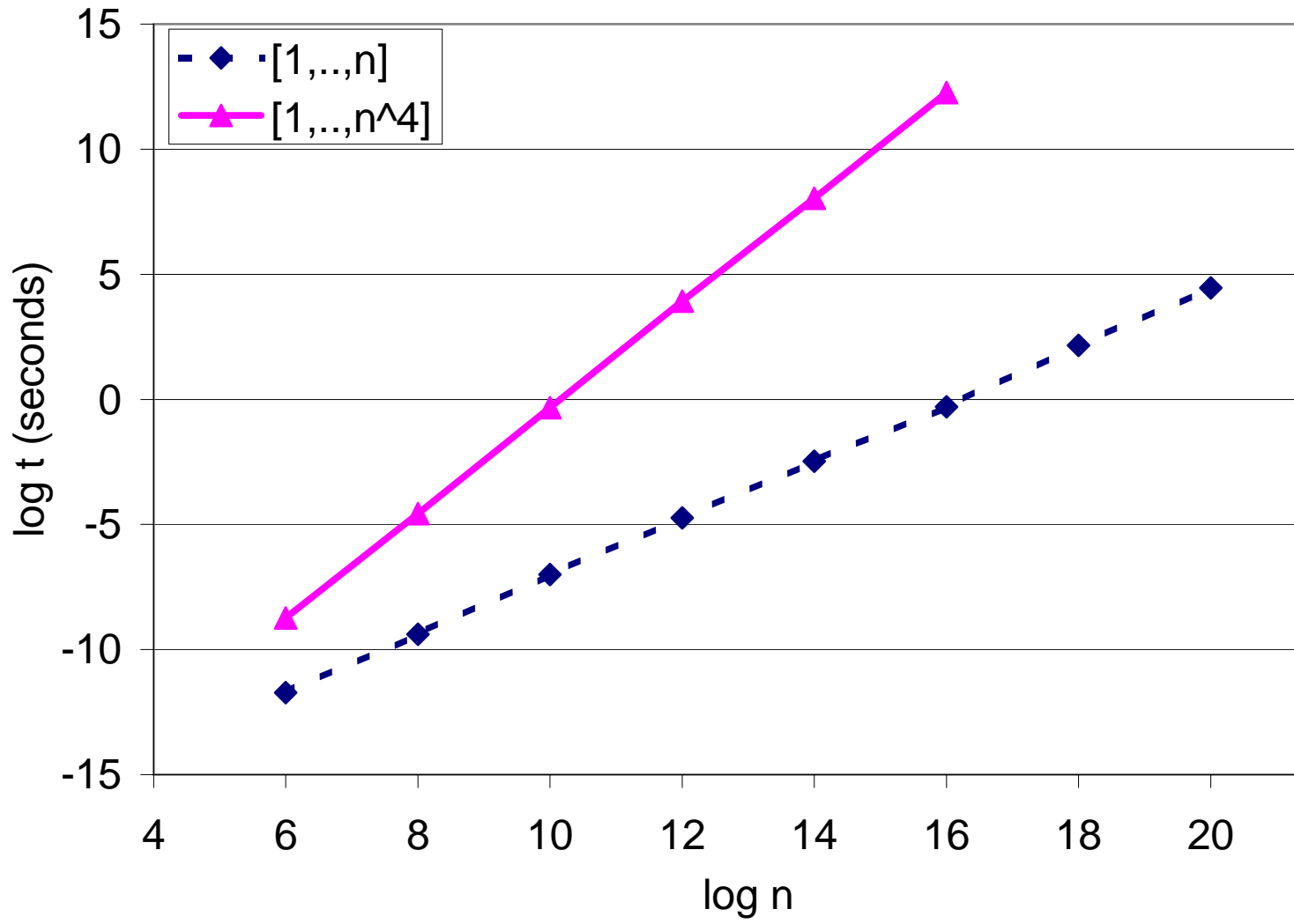
Running Time vs. Input Size
