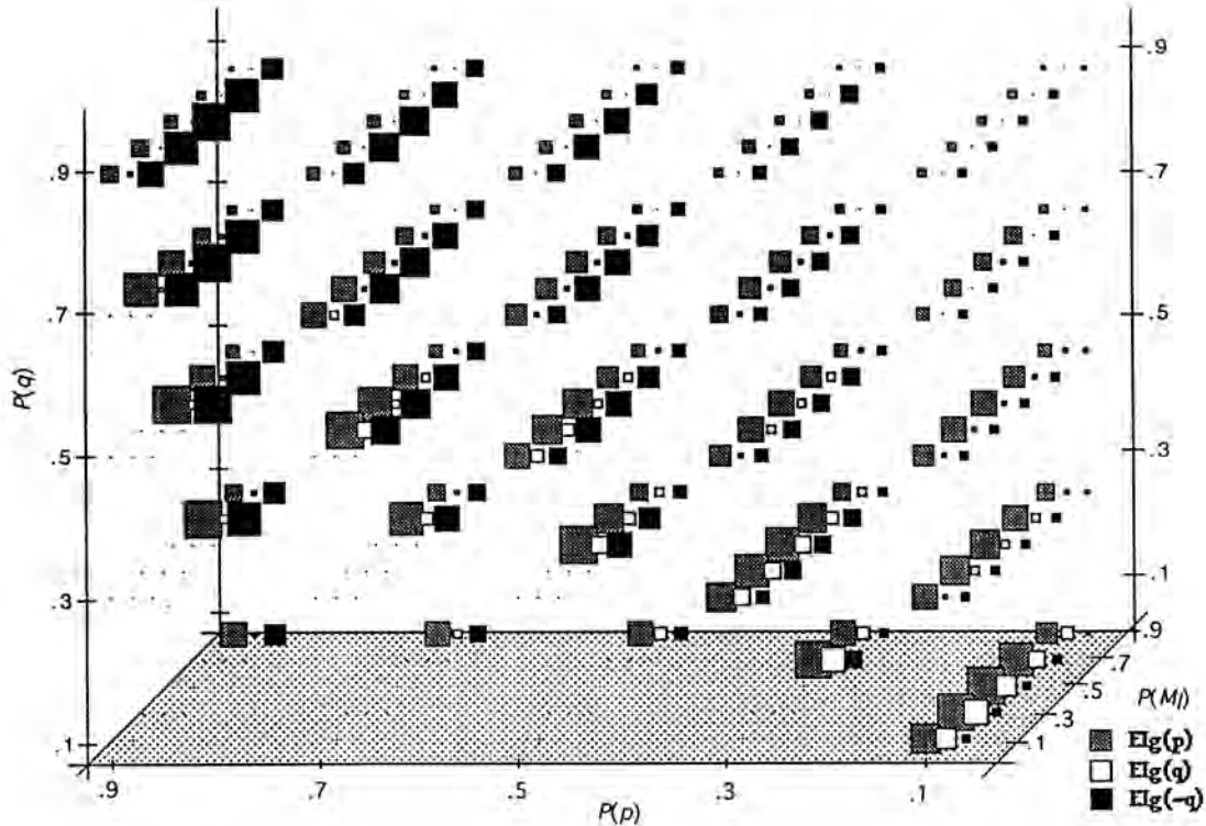
Figure 2. Model behavior. At each [P(p), P(q), P(M_I)] coordinate, the three boxes represent the E(I_r) values for the three cards. The area of the box is proportional to the E(I_r) for the corresponding card. Coordinates where there are three dots indicate regions where the inequality P(q) \geq P(q)P(M_D) is violated, and hence the probability values are inconsistent. M_I = independent model.
