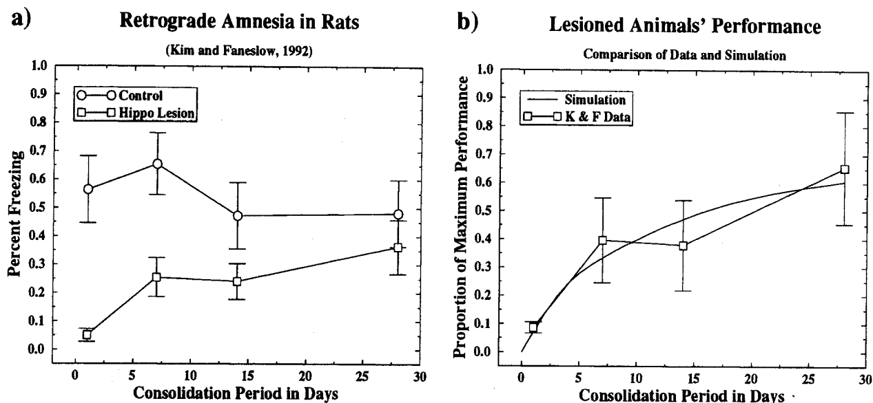
Figure 12. Consolidation in the experiment of Kim and Fanselow (1992). Panel a: Experimental data from experimental and control groups. Panel b: Simulation of consolidation in the group with hippocampal lesions. Panel b shows the experimental data with error bars, together with a curve describing the buildup of performance over the consolidation in the simulation. In this panel, the measure used for the experimental data is the amount of time spent freezing for each experimental group divided by the average amount of time spent freezing across the control groups at different delays. The measure used for the simulation divides the reduction in output mean squared error at each test point by the initial amount of error to the test input before any learning on this pattern. Note. Data in Panel a are from "Modality-Specific Retrograde Amnesia of Fear," by J. J. Kim and M. S. Fanselow, 1992, Science , 256, p. 676. Copyright 1992 by the American Association for the Advancement of Science. Reprinted with permission.
